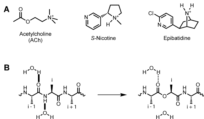
Figure 3. (A) Structures of agonists considered here. (B) The backbone ester strategy for modulating hydrogen bonding interactions.
