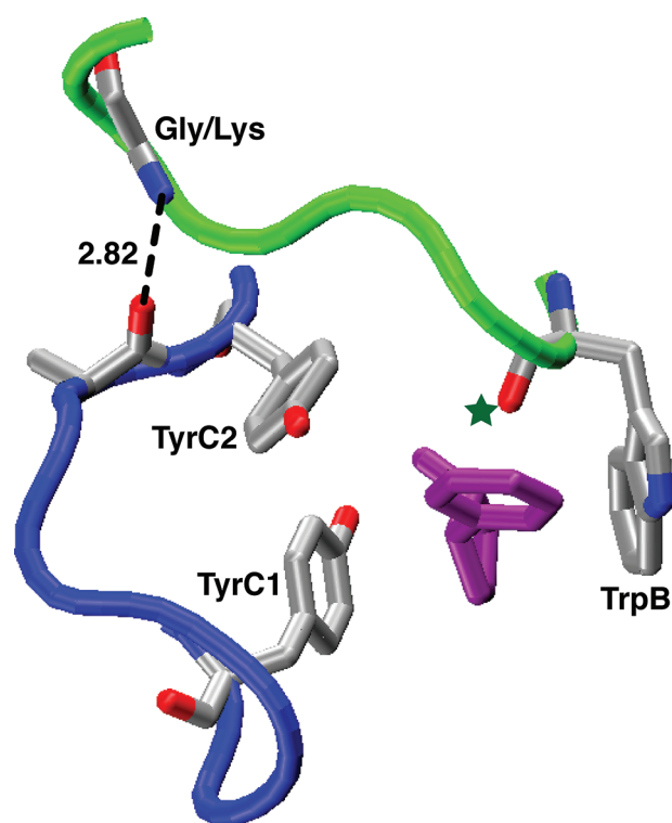
Figure 2. Image of the nAChR agonist binding site, based on the structure of AChBP with nicotine bound (PDB id: 1UW6). 20 Loop B is in green, and loop C is in blue. Three of the five residues that form the “aromatic box” of the agonist binding site are shown, and nicotine is shown in purple. A green star marks the backbone carbonyl that hydrogen bonds to the N + H of agonists, and the proposed loop B–loop C hydrogen bond that is a major focus of the present work is highlighted.
